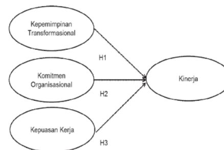
Gambar 1. Model Penelitian
